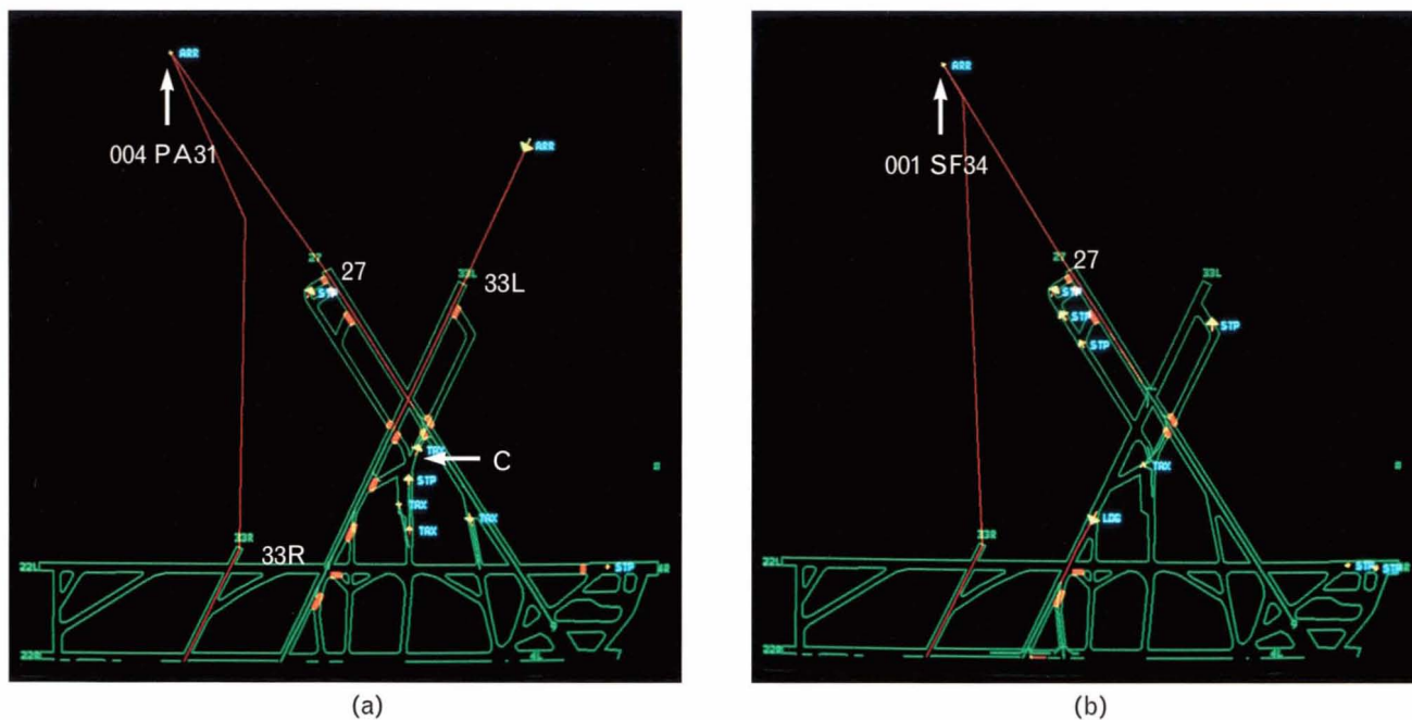
FIGURE 9. Ambiguous projection of landing aircraft. (a) A Piper Navajo (PA31) is on approach to Runway 33R but projected to both Runways 33R and 27. The surface monitor chooses the primary runway based on the traffic flow in the current runway configuration and illuminates the runway-status lights accordingly. In this case the primary runway was Runway 27; hence the RELs illuminated along that runway. The correct, unambiguous projection was established on the next scan of the radar and the RELs along Runway 27 turned off. A little later, as the aircraft's hot zone reached Runway 33R, the RELs along that runway illuminated normally. (b) This approach was flown two minutes after the approach shown in part a. Again there is an ambiguous projection, but this time the aircraft, a Saab/Fairchild 340 (SF34), did indeed land on Runway 27, so the primary projection was correct.
