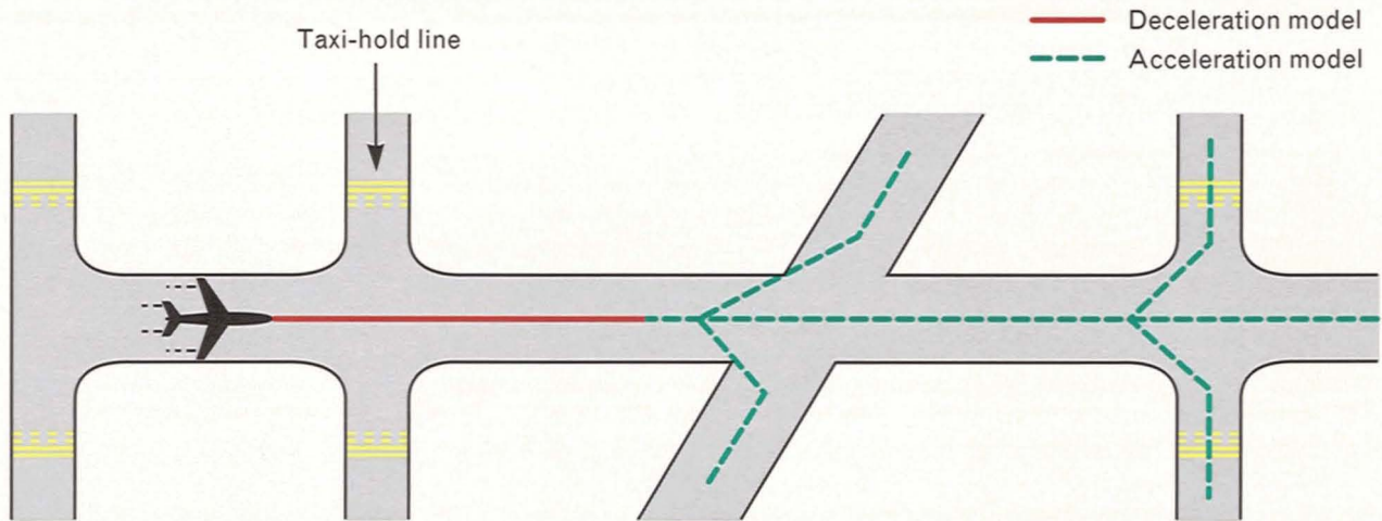
FIGURE 3. Path-prediction trees. The prediction engine computes two sets of predicted paths that show where a target could be in the future, based on two models of target motion, which are functions of target state. One model, called the acceleration model, assumes the target will travel as far as reasonable within a given look-ahead time; its predicted path is represented by the dashed green lines. The other model, called the deceleration model, assumes the target is attempting to stop (but not a panic stop) within a given look-ahead time; its predicted path is represented by the solid red line (the red line is superimposed on the dashed green line). Thus the two sets of predicted paths, or trees , compute reasonable bounds on future target position.
