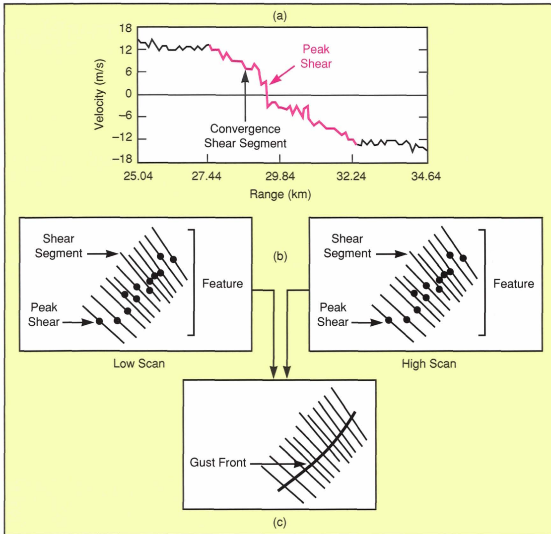
Fig. 12—Diagram illustrating gust front detection. (a) Radial-velocity data are searched for segments of decreasing Doppler velocity, which indicates radial convergence. The dots represent the locations of the peak shears along each segment. (b) Segments from the low (0.5) and high (1.0) tilts are grouped respectively into features, and (c) features are grouped on the basis of spatial proximity into gust fronts.
